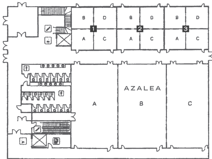
2nd FLOOR
